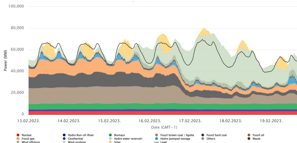
Chart 2. Electricity generation changes in one week in Germany in February 2023
