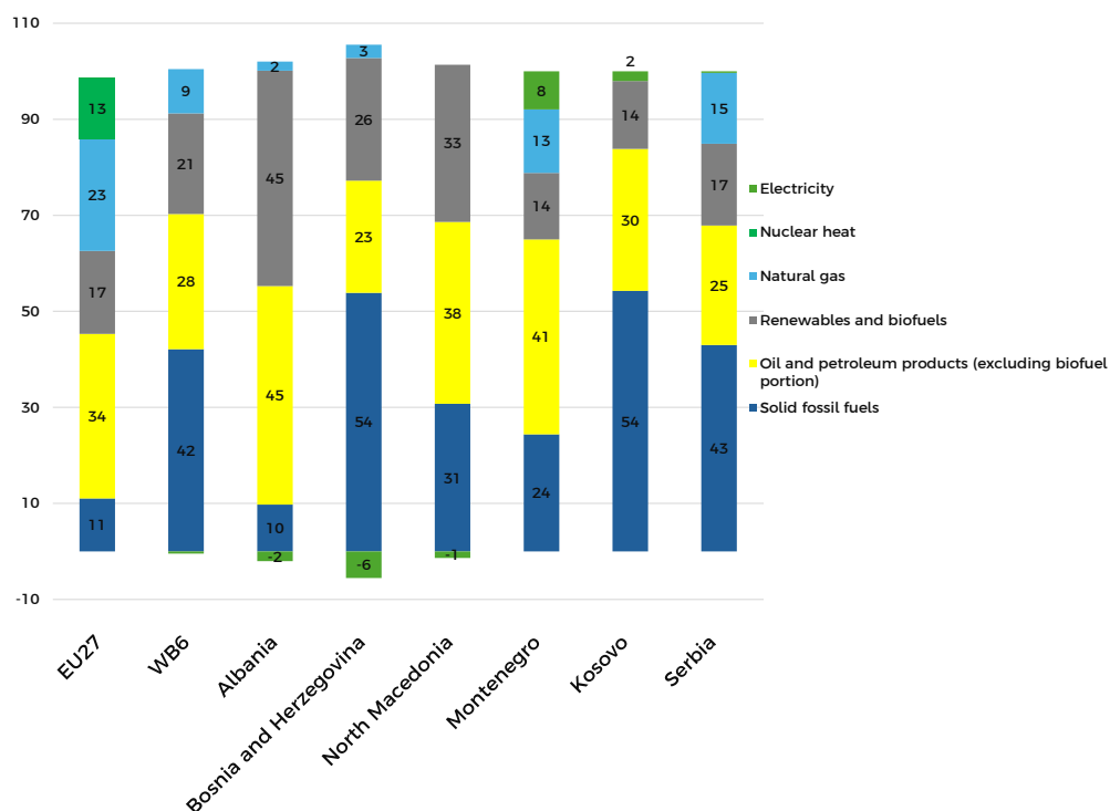
Chart 7. Gross available energy in the WB6 and the EU27 by fuel types - 2021 (%)
